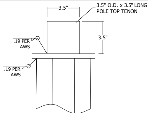
DETAIL 1 - POLE TOP TENON
