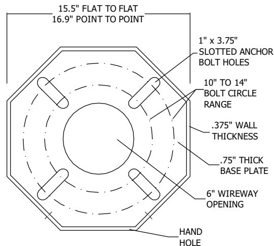
DETAIL 3 - BASE PLATE
