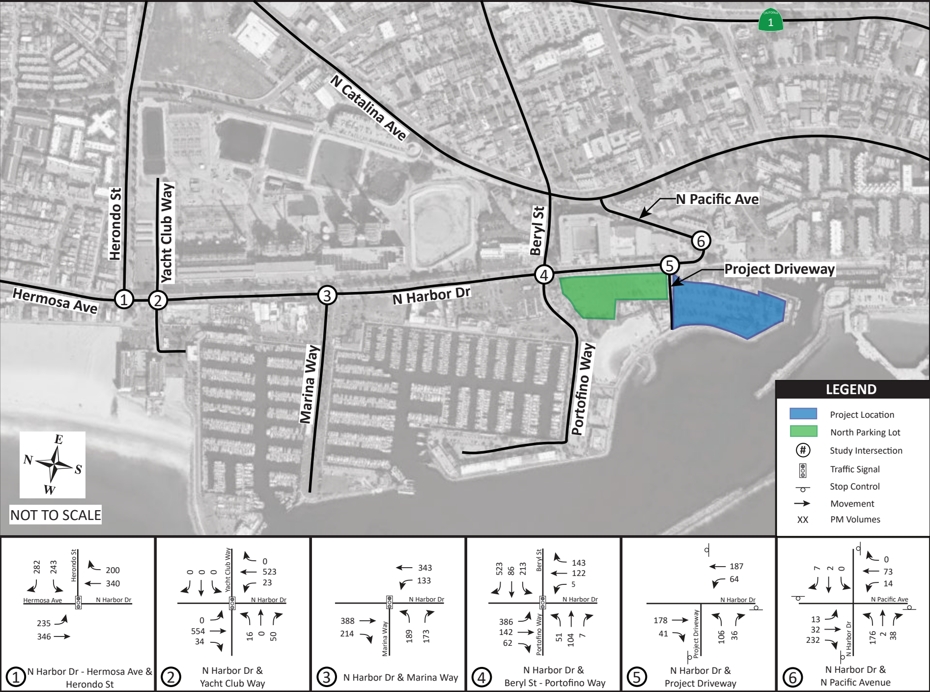
Figure 2-11 Opening Year 2027 With Project PM Peak Hour Intersection Volumes
