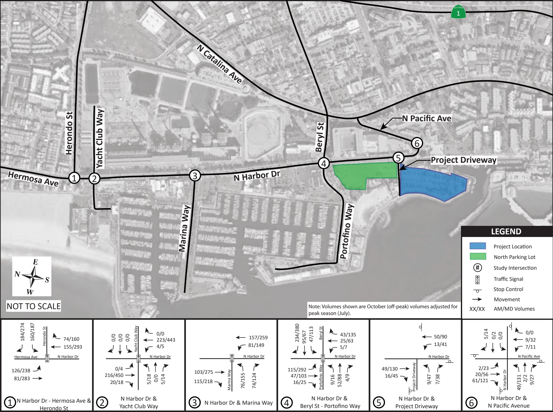
Figure 2-3 Existing AM and MD Peak Hour Intersection Volumes
