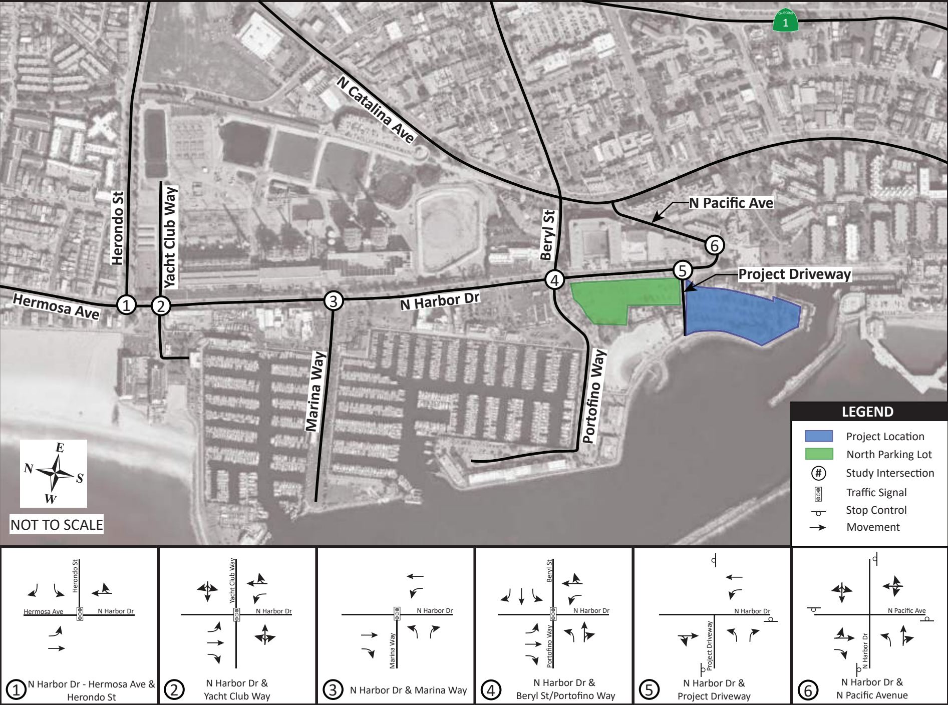
Figure 2-2 Existing Intersection Geometry
