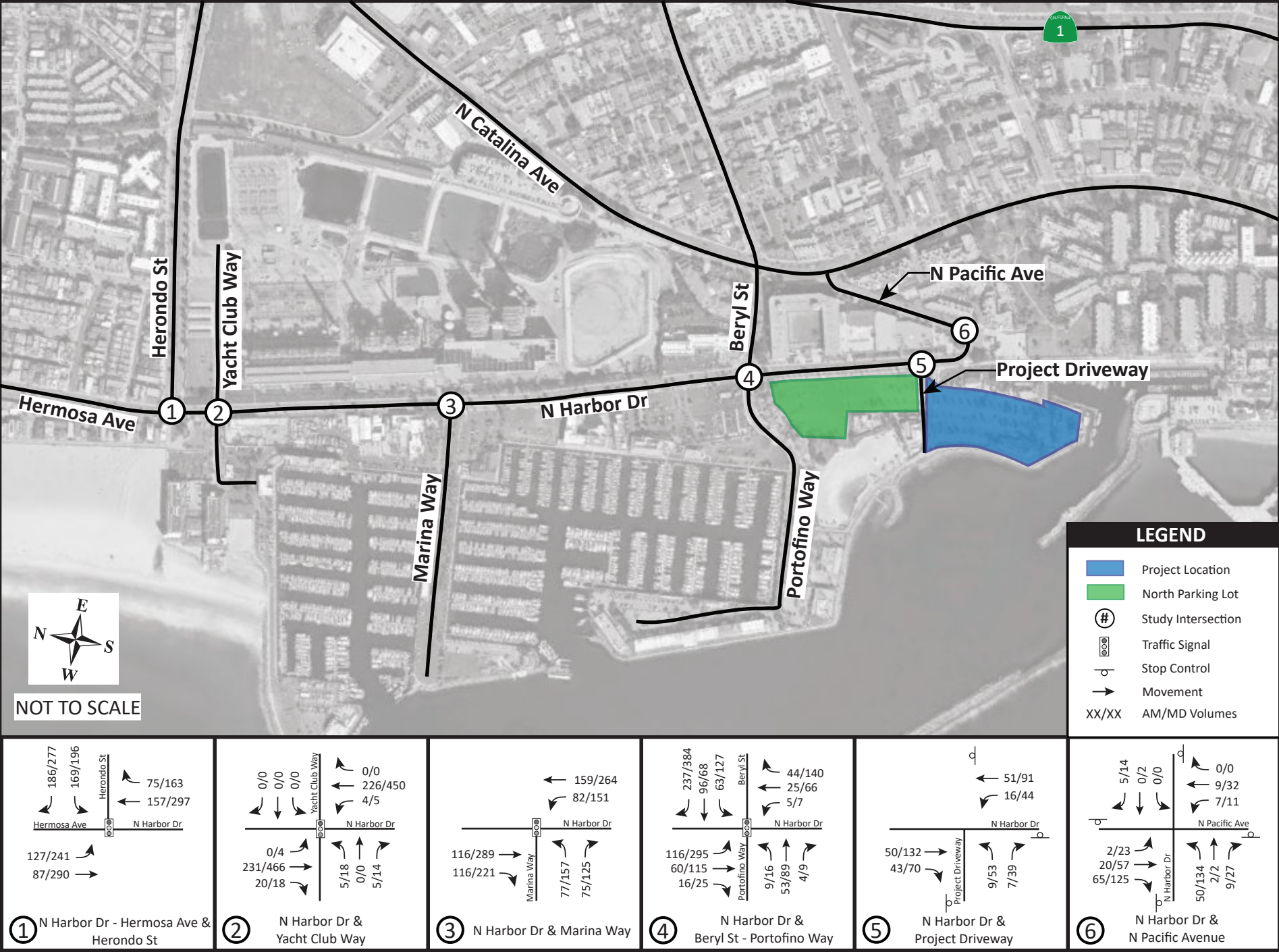
Figure 2-10 Opening Year 2027 With Project AM and MD Peak Hour Intersection Volumes
